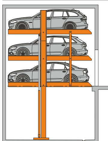
System lifted
