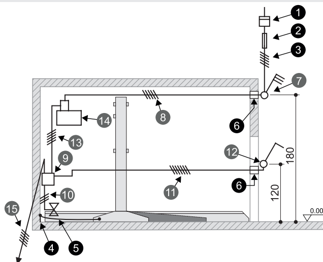
Electrical installation diagram
