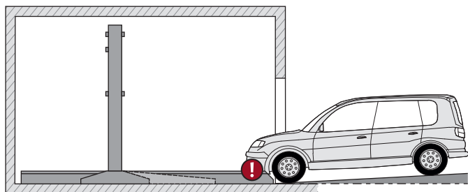
max. 4% slope
