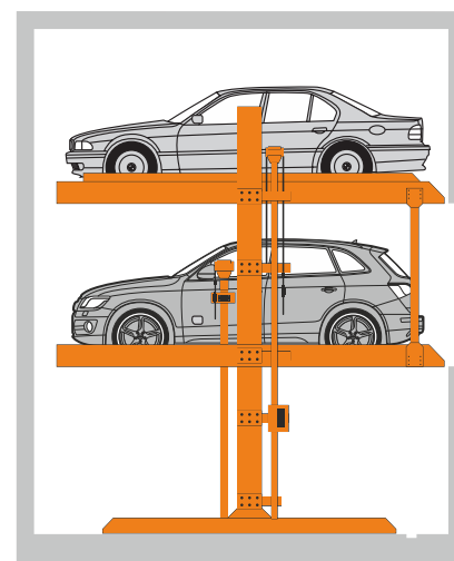
UG platform at entry level
