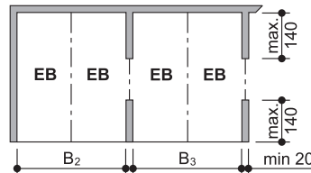
Double arrangement (2 x EB)
